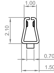
Sec:C-C
